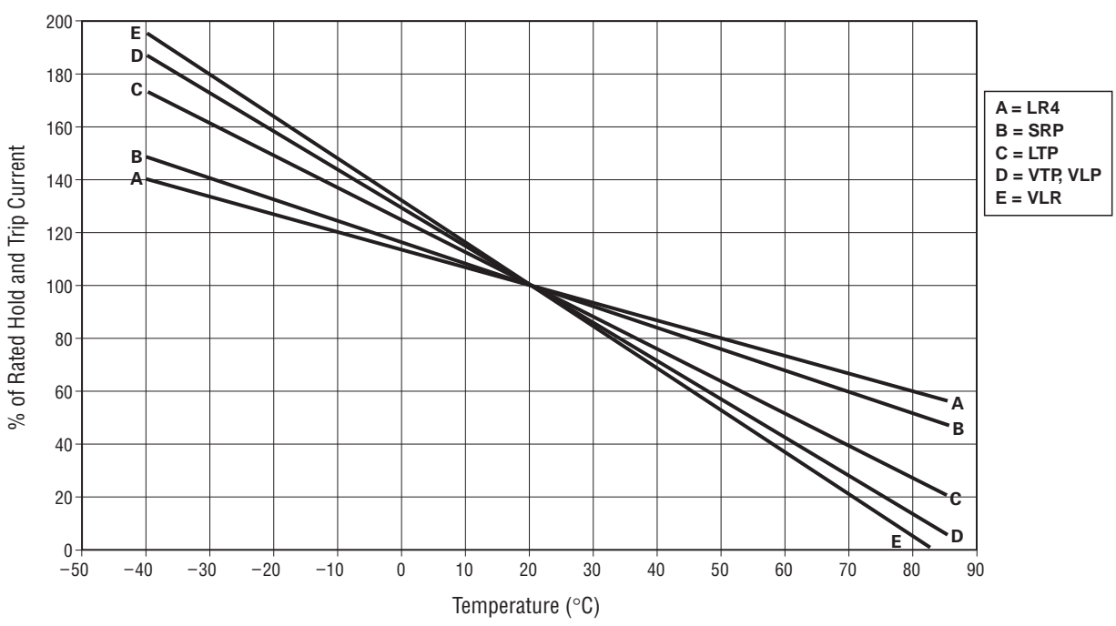
Figure B1 - Thermal Derating Curve
